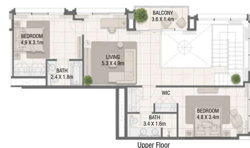
Upper Floor
